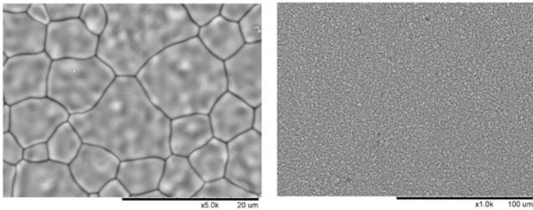
Fig. 1~2 The surface and fraction of 8YSZ electrolyte
